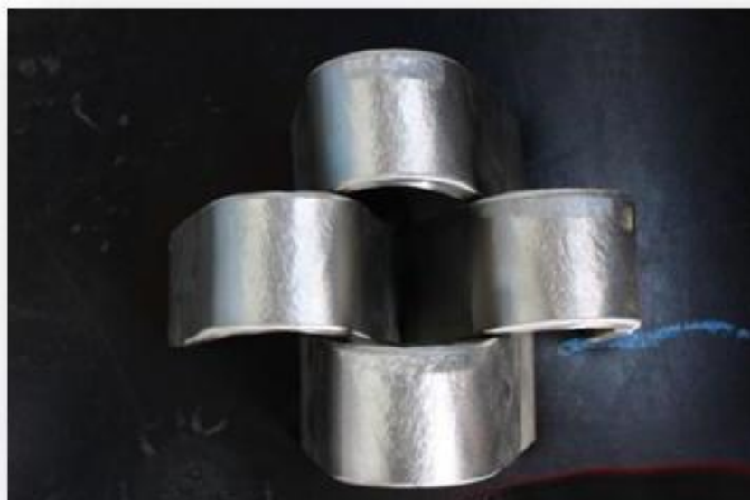
Figure 19. 2 inch (50.8mm) full section p-GMAW 2T side bend tests.
